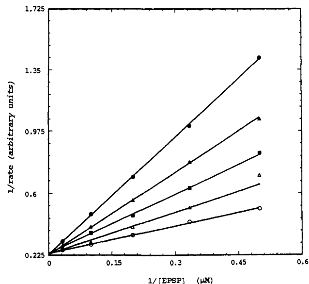
Figure 1. Lineweaver-Burk plot for inhibition of EPSP synthase by isomer 2r in competition with EPSP: [\text{P}_i] = 50 \text{ mM} , [\mathbf{2r}] = 0 ( \circ ), 6 nM ( \Delta ), 10 nM ( \blacksquare ), 25 nM ( \blacktriangle ), and 50 nM ( \bullet ). Each point represents an average of two or three determinations; the data were fit using Cleland's COMP program. 19
